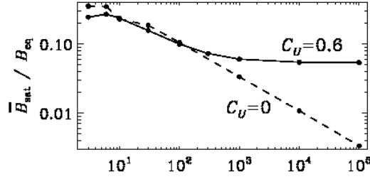
Figure 21: Saturation magnetic energy normalized for equipartition versus magnetic Reynolds number \text{Re}_M with advective helicity flux (solid line). Compare the case without the flux (dashed line). The catastrophic quenching gets alleviated by helicity fluxes.
