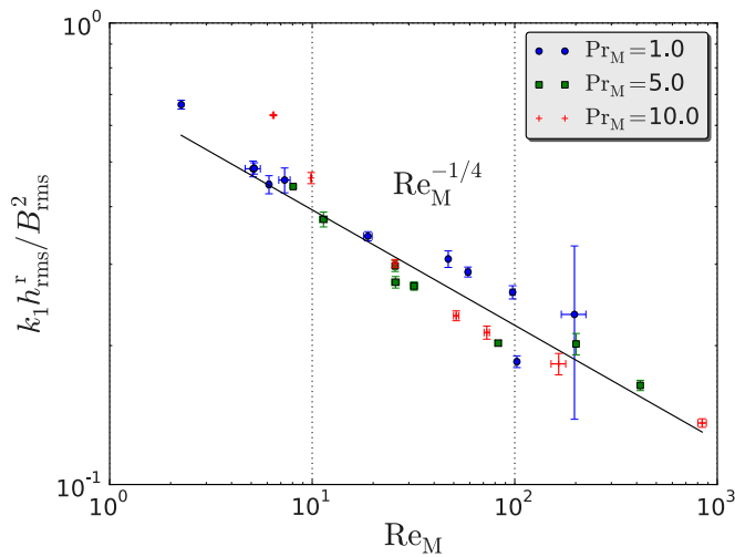
FIG. 6. (Color online) \text{Re}_M dependence of k_1 h_{\text{rms}}^r / B_{\text{rms}}^2 for the kinematic phase. Values are averages over times where they reach a stationary state. A -1/4 power law can be seen.
