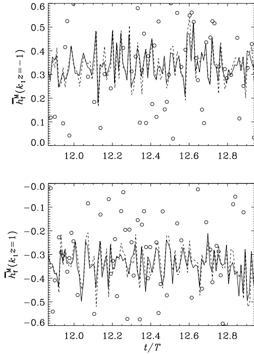
Fig. 4 Plot of \overline{h}_f^M as a function of time in the statistically stationary state for k_1 z = -1 (south, top panel ) and k_1 z = 1 (north, bottom panel ) for the three different gauges, Weyl gauge (open circle), Lorenz gauge (line) and resistive gauge (broken line).
