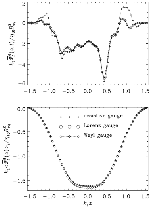
Fig. 5 Comparison of the flux \overline{\mathcal{F}}_f^H(z, t) at a randomly chosen instant ( upper panel ) and its time average \overline{\mathcal{F}}_f^H(z) for the three different gauges. Lorenz gauge ( \circ ), Weyl gauge ( \diamond ) and the resistive gauge ( \cdot ). The instantaneous flux is plotted in the top panel and the time-averaged flux is plotted in the bottom panel.
