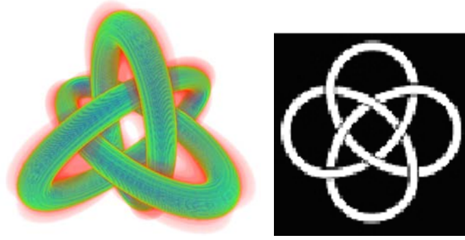
Figure 29: Left: Borromean rings. Right: IUCAA logo.
