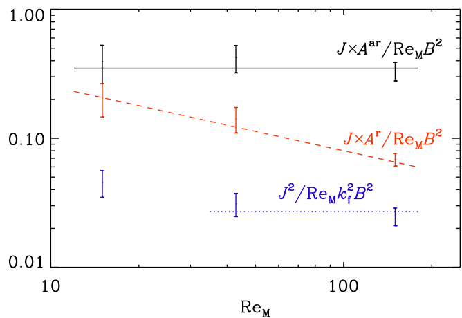
FIG. 8. (Color online) \text{Re}_M scaling of the rms value of \mathbf{J} \times \mathbf{A} , normalized by \text{Re}_M B_{\text{rms}}^2 , for the advecto-resistive and resistive gauges. The solid line represents constant scaling, i.e., \eta \mathbf{J} \times \mathbf{A}^{\text{ar}} \approx \text{const} , while the dashed line represents inverse square root scaling, i.e., \eta \mathbf{J} \times \mathbf{A}^r \propto \text{Re}_M^{1/2} , for three runs with \text{Pr}_M=1 in the saturated regime. The dotted/blue line shows that \eta J^2 , properly normalized, is approximately constant.
