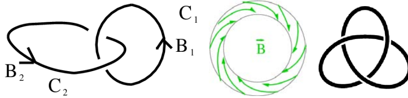
Figure 11: Left : Two interlocked flux rings which make up a helical configuration. Center : Magnetic flux ring which has a twisted magnetic field and finite helicity. Right : The trefoil knot [Moffatt, 1969]. With a magnetic field tangential to the knot the helicity of the configuration is finite.
