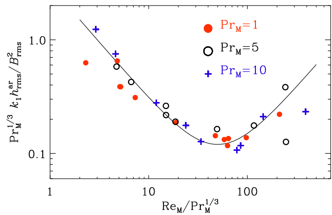
FIG. 7. (Color online) Dependence of k_1 h_{\text{rms}}^{\text{ar}} / B_{\text{rms}}^2 , scaled by \text{Pr}_M^{1/3} on \text{Re}_M / \text{Pr}_M^{1/3} for the kinematic phase and \text{Pr}_M=1 (filled circles), 5 (open circles), and 10 (plus signs). The solid line represents the fit of Eq. (25).
